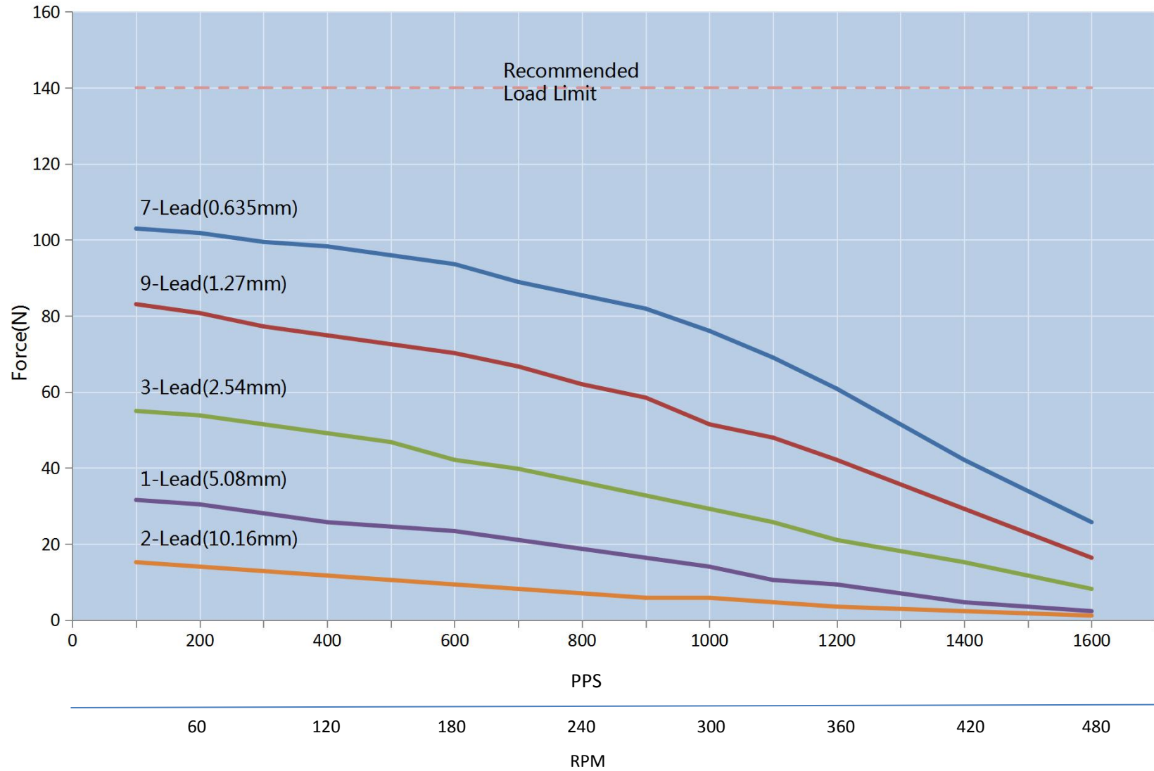
Nema 11 linear steppers double stack(24V)
