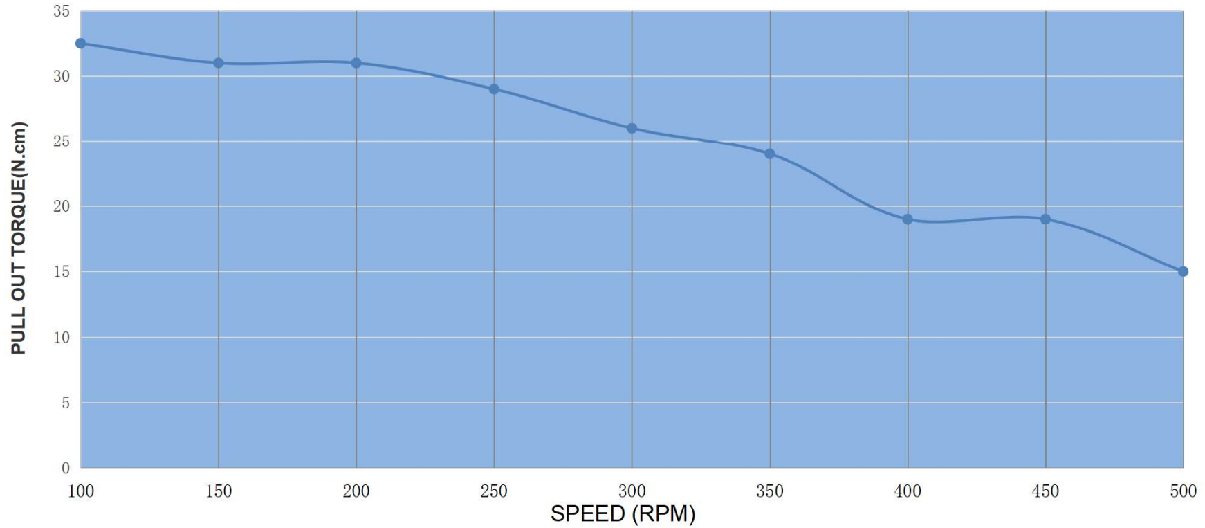
PULL OUT TORQUE CURVE OF 17HS15-1584S
